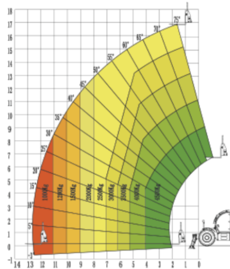
Outrigger Down
