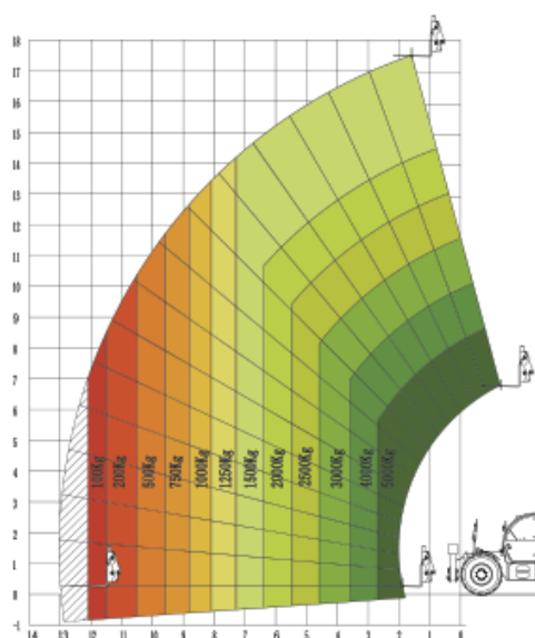
Outrigger Up
