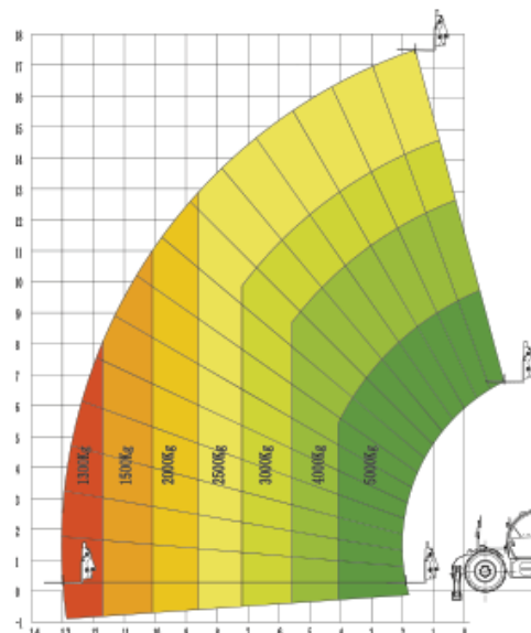
Outrigger Down
